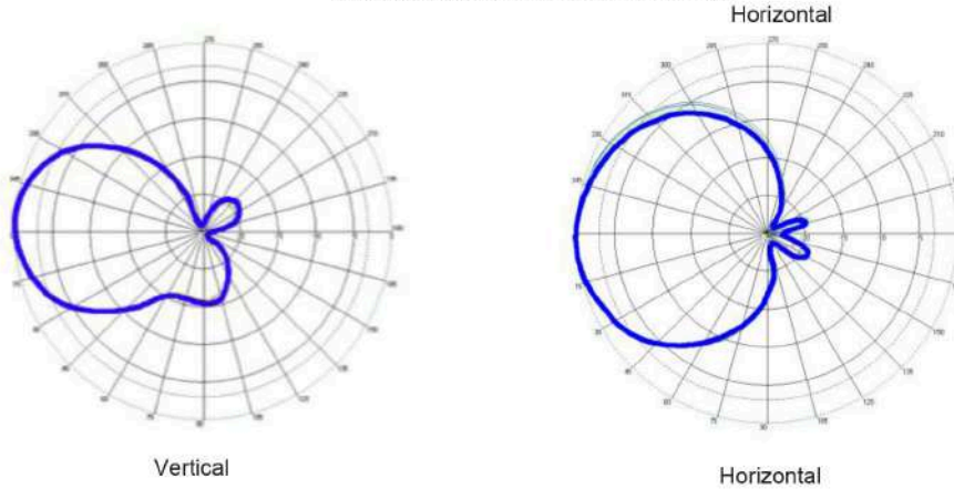
E-field elevation & Azimuth Patterns
