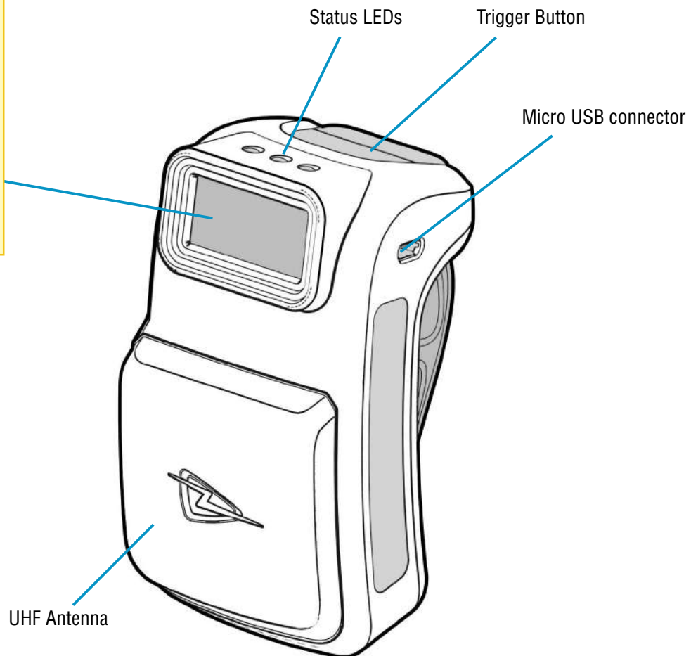
FIGURE 1: Parts of the 1153 UHF Reader
