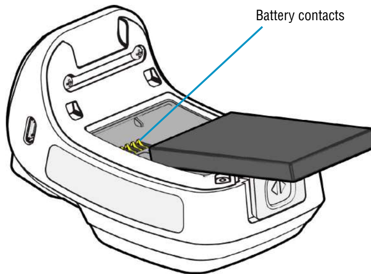
FIGURE 6: Battery placement
